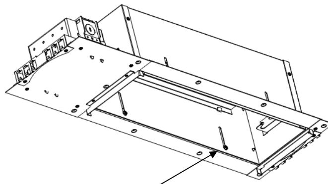
Housing shell screws (2 each side)
