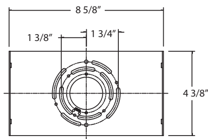
Mounting Backplate
