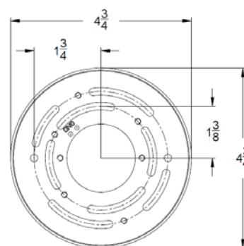
PD-58908 Back Ring Dimensions
