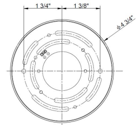
Mounting Ring Dimensions
